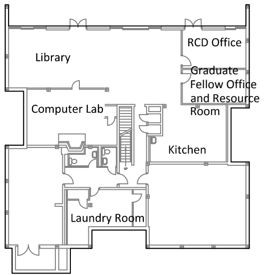
HURD GROUND FLOOR
